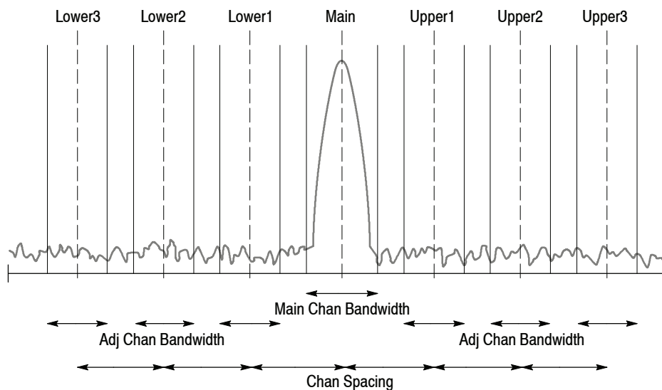
Figure 3-5: ACPR measurement band power markers
