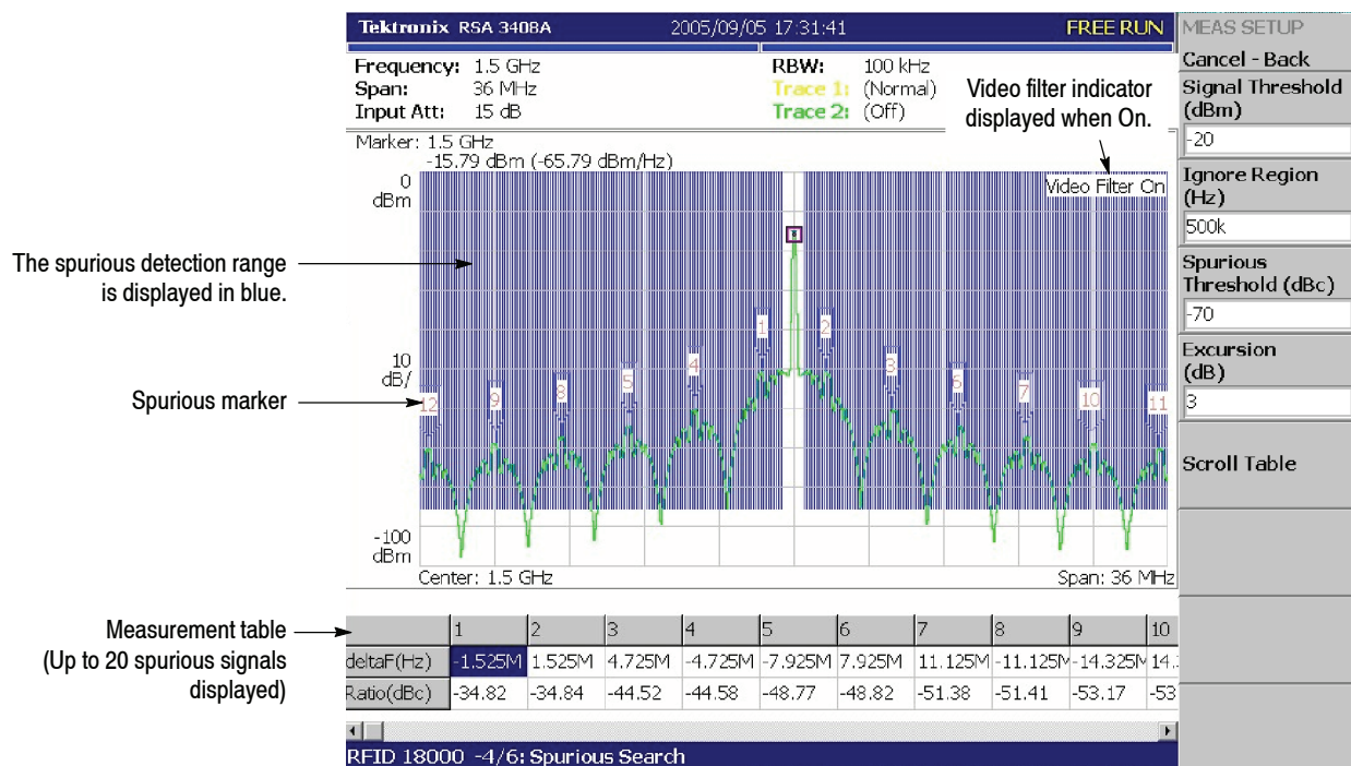
Figure 3-65: Spurious measurement
