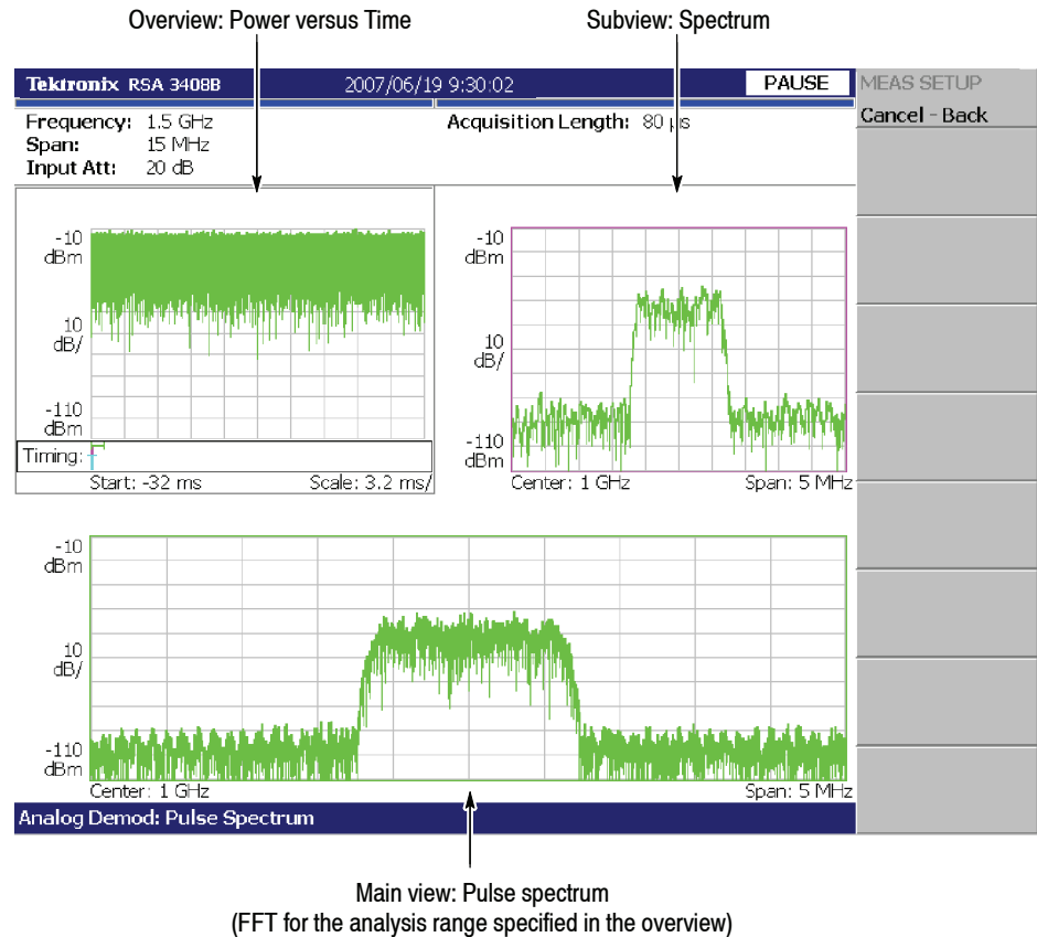
Figure 3-43: Pulse spectrum measurement
