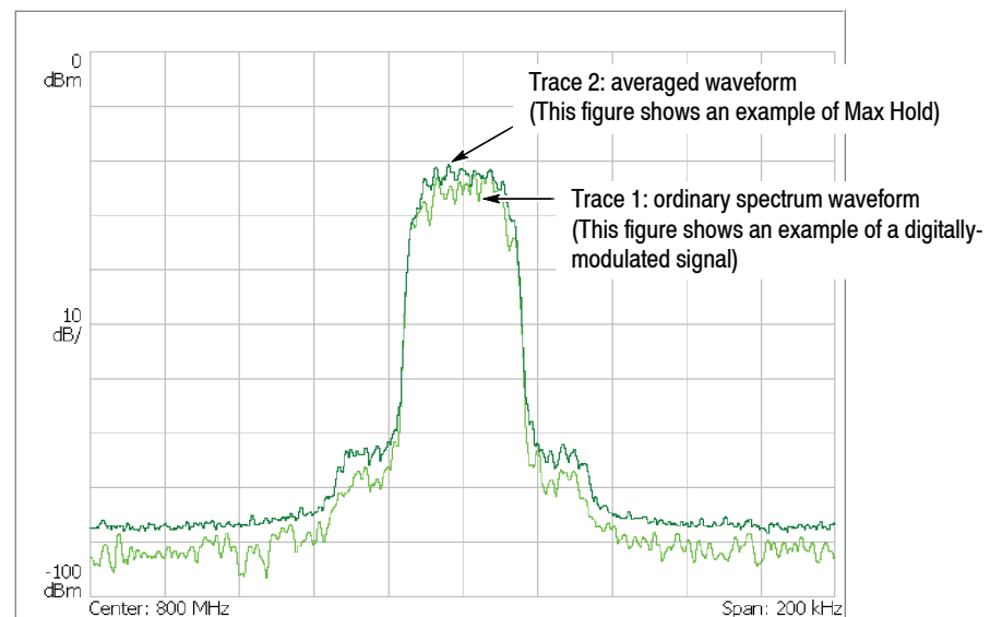
Figure 3-137: Compared display
