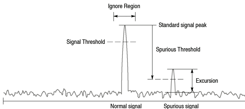
Figure 3-14: Setting up spurious signal measurement
