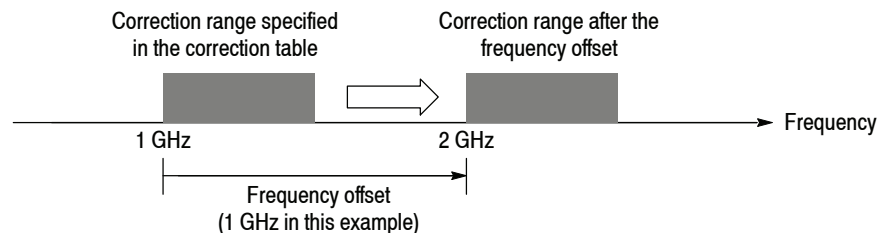
Figure 3-107: Frequency offset
