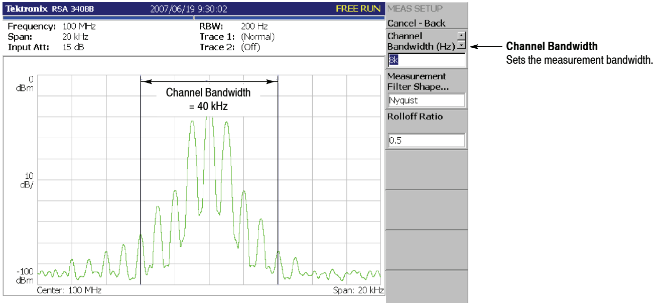
Figure 2-49: Channel power measurement (Channel Bandwidth = 40 kHz)
